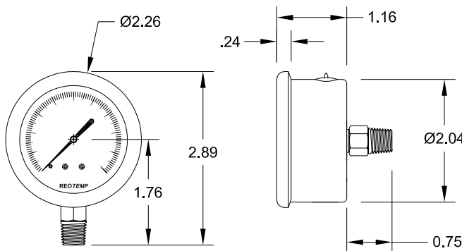
PG20 *dimensions in inches
